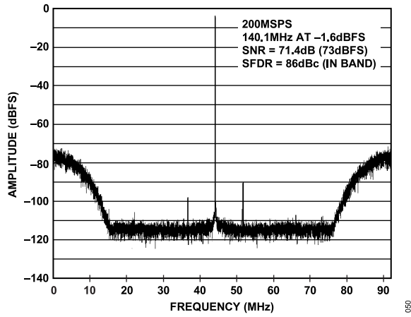
Figure 57. 33% BW Mode, Tuning Word = 17 ( f_s/4 Tuning)
