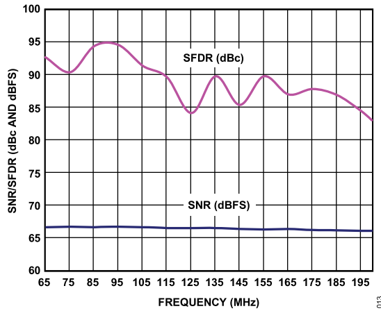
Figure 13. AD6643-200 Single Tone SNR/SFDR vs. Input Frequency ( f_{IN} )
