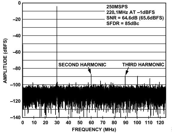
Figure 24. AD6643-250 Single Tone FFT, f_{IN} = 220.1 MHz
