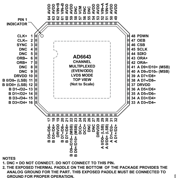
Figure 5. Pin Configuration (Top View), LFCSP Channel Multiplexed (Even/Odd) LVDS
