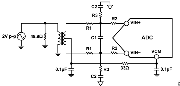
Figure 43. Differential Transformer-Coupled Configuration
