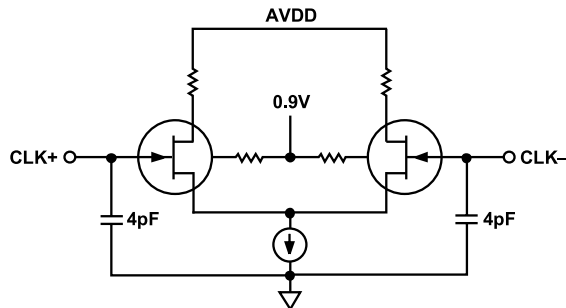
Figure 46. Equivalent Clock Input Circuit
