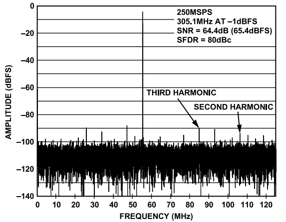
Figure 25. AD6643-250 Single Tone FFT, f_{IN} = 305.1 MHz
