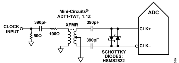
Figure 47. Transformer-Coupled Differential Clock (Up to 200 MHz)
