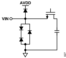
Figure 34. Equivalent Analog Input Circuit
