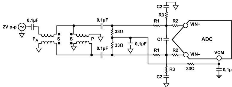
Figure 44. Differential Double Balun Input Configuration
