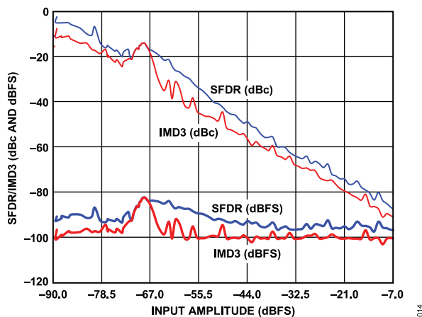
Figure 14. AD6643-200 Two Tone SFDR/IMD3 vs. Input Amplitude ( A_{IN} ) with f_{IN1} = 89.12 MHz, f_{IN2} = 92.12 MHz
