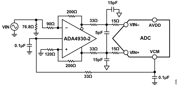
Figure 42. Differential Input Configuration Using the ADA4930-2
