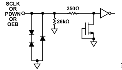
Figure 38. Equivalent SCLK or PDWN or OEB Input Circuit
