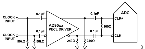
Figure 49. Differential PECL Sample Clock (Up to 625 MHz)
