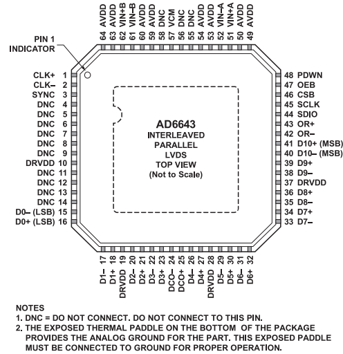
Figure 4. Pin Configuration (Top View), LFCSP Interleaved Parallel LVDS
