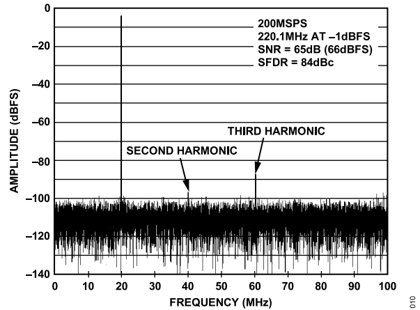
Figure 10. AD6643-200 Single Tone FFT, f_{IN} = 220.1 MHz
