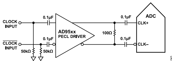
Figure 50. Differential LVDS Sample Clock (Up to 625 MHz)
