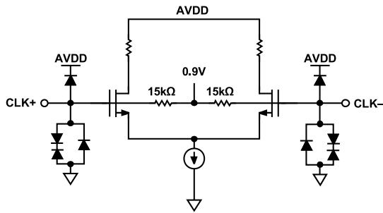
Figure 35. Equivalent Clock Input Circuit
