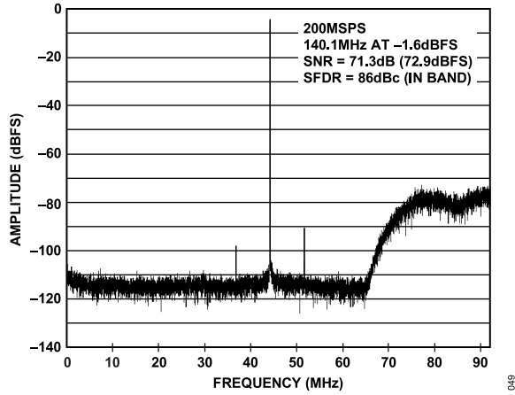
Figure 56. 33% BW Mode, Tuning Word = 5
