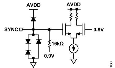
Figure 40. Equivalent SYNC Input Circuit
