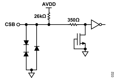
Figure 39. Equivalent CSB Input Circuit
