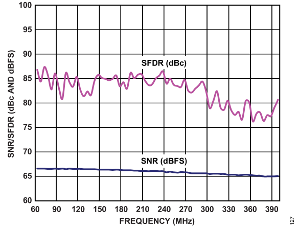
Figure 27. AD6643-250 Single Tone SNR/SFDR vs. Input Frequency ( f_{IN} ), V_{REF} = 1.75 V p-p
