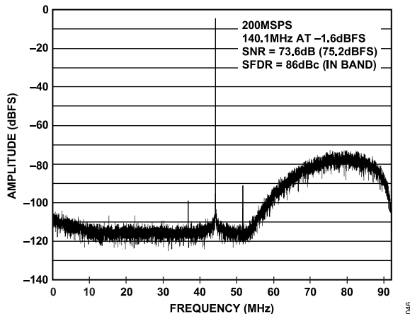
Figure 53. 22% BW Mode, Tuning Word = 13
