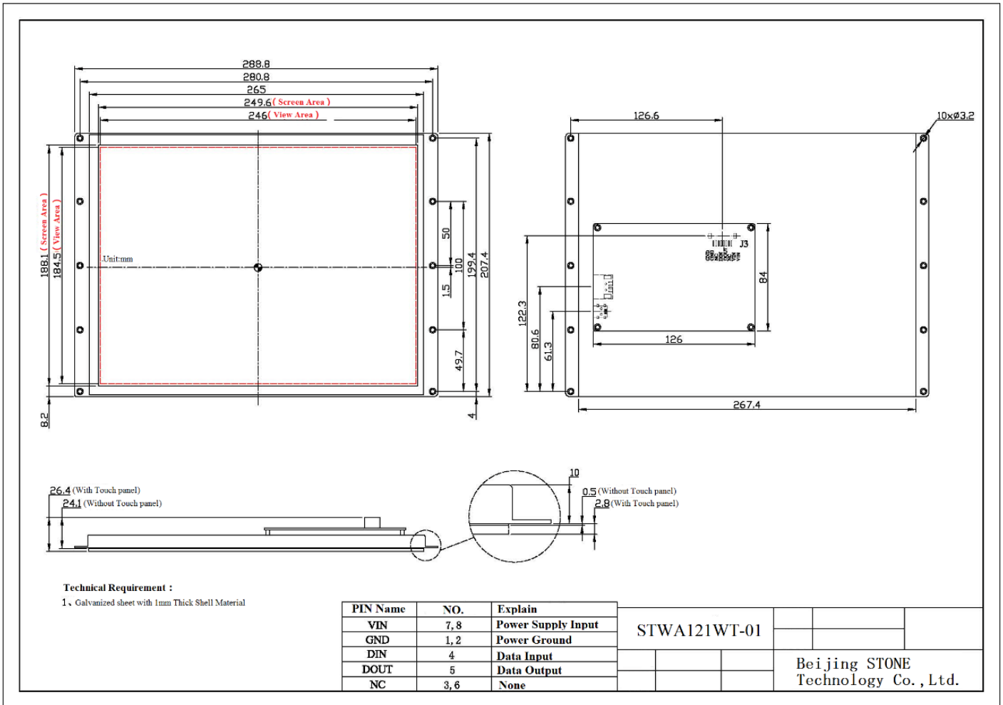
Figure 6-1 STWA121WT-01 dimension
